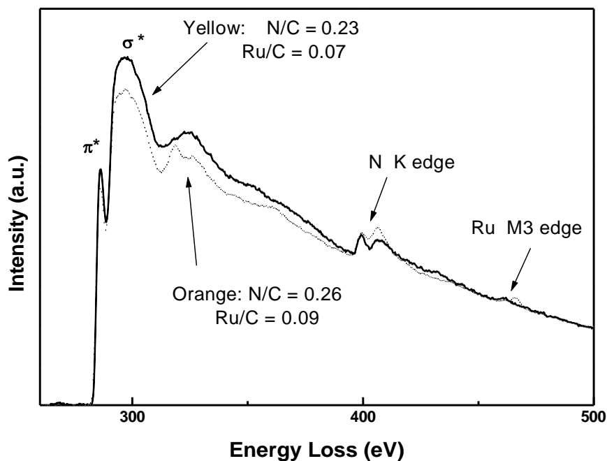
Figure 4. High-energy loss region of EELS spectra showing the K ionization edges from C and N and Ru M 3 edge of yellow (continuous) and orange (dotted) samples.
