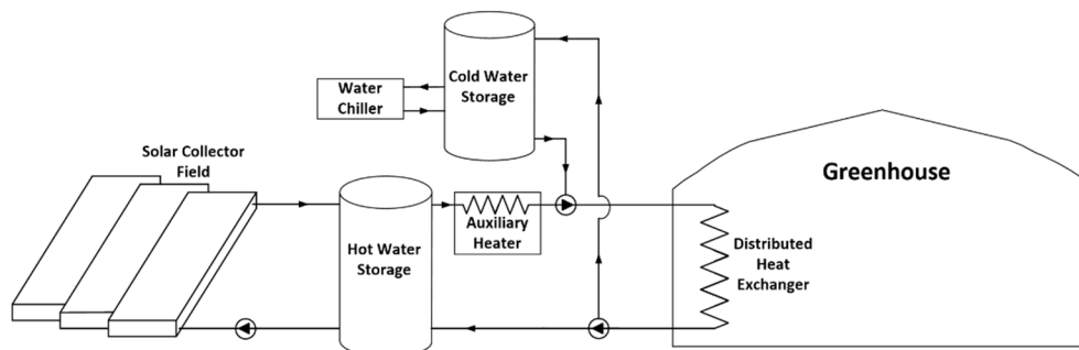
Fig. 3: Greenhouse air conditioning system proposed.
