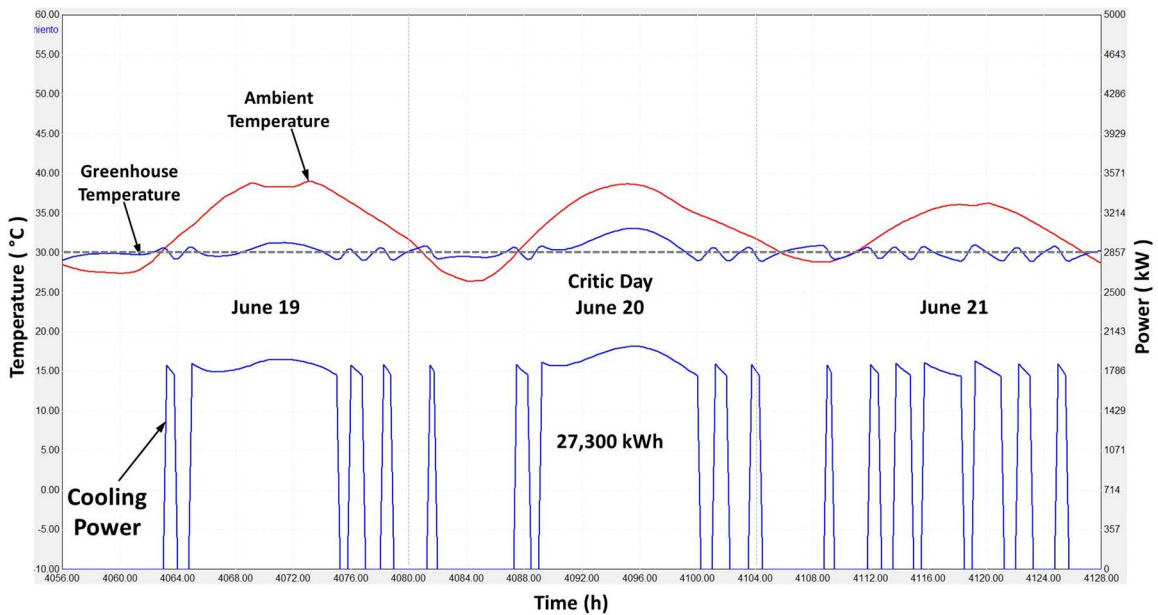
Fig. 12: Thermal performance inside and outside the greenhouse using air conditioning on June 19th, 20th and 21st.
