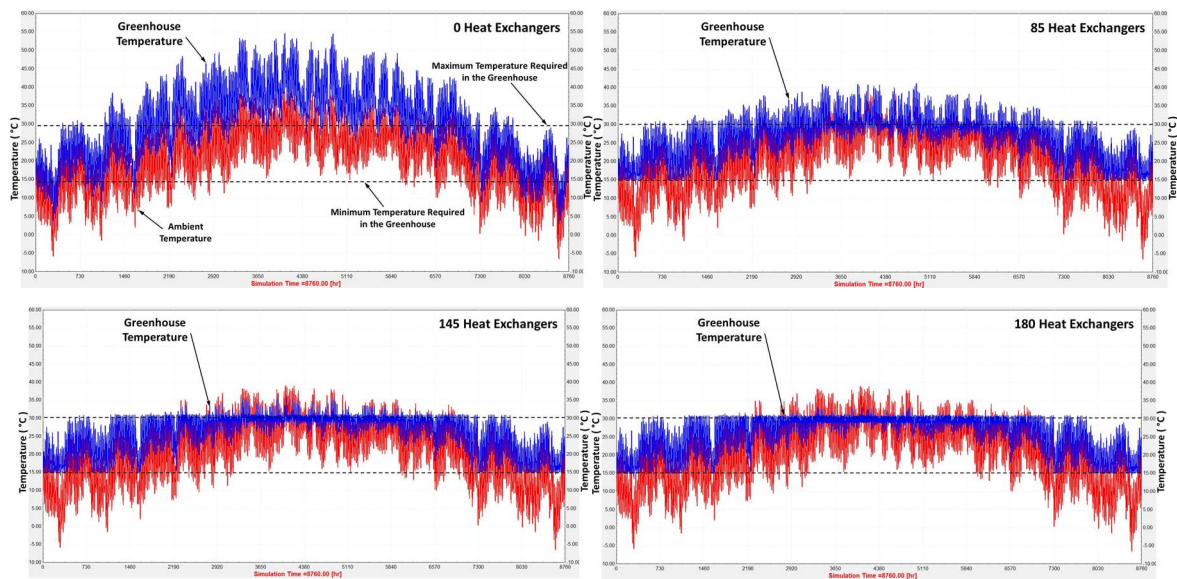
Fig. 9: Thermal performance in the greenhouse using 85, 145 and 180 heat exchangers.
