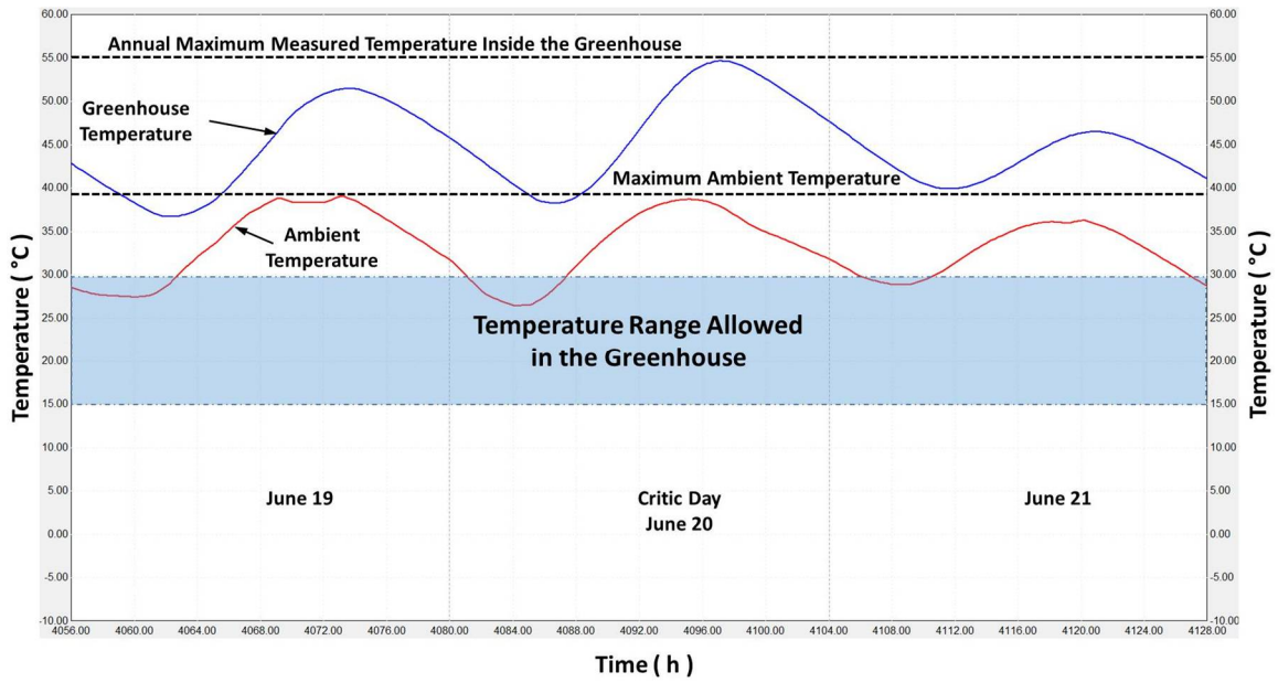
Fig. 11: Temperatures reached inside and outside the greenhouse on June 19th, 20th and 21st.
