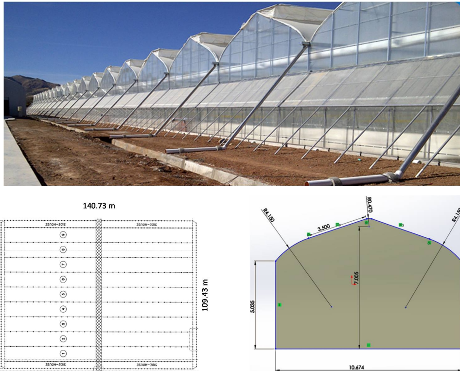
Fig. 2: Multi-chapel Greenhouse type
