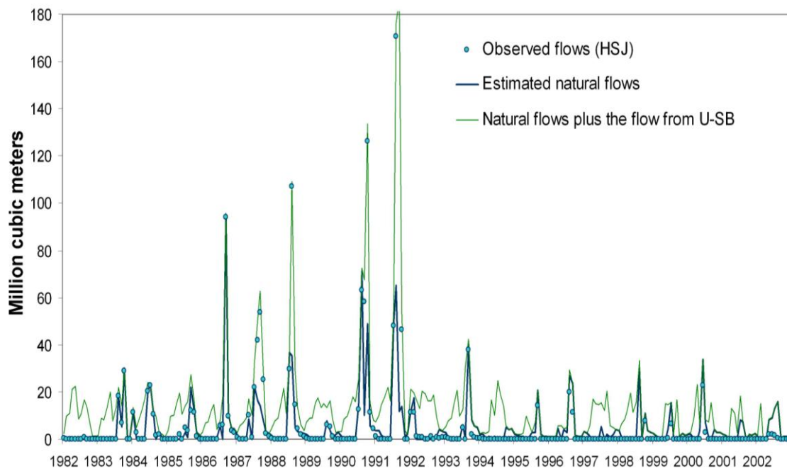
Figure 5. Monthly natural flow estimated from 1982 to 2002 at the exit of sub-basin M-SB, historical flow gauged at the Jiménez Hydrometric Station, and natural flow plus the flow from sub-basin U-SB.
