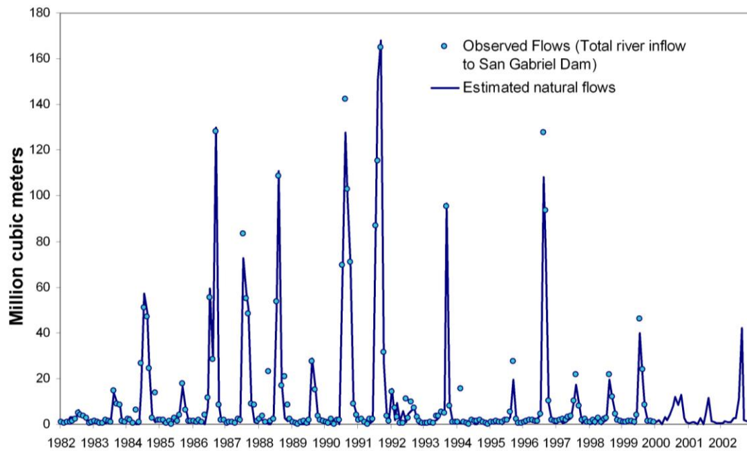
Figure 4. Natural flow estimated from 1982 to 2002 at the exit of U-SB, and total river inflow to San Gabriel Dam of the NSWDB (IMTA and CNA, 2000).
