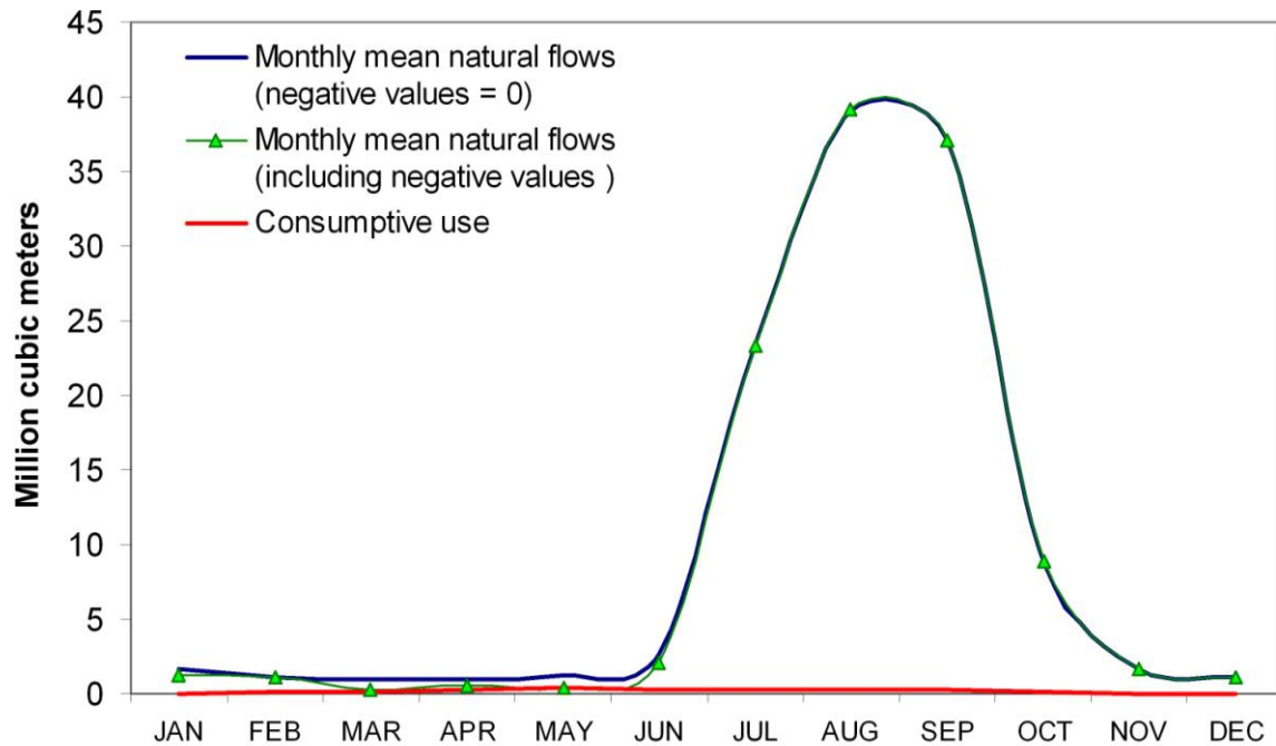
Figure 2. Natural flow and monthly consumptive use from 1982 to 2002
