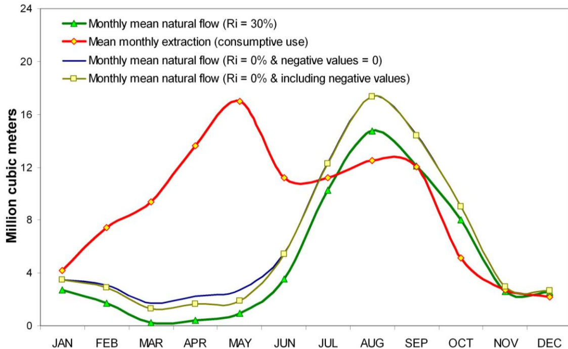
Figure 3. Natural flow and monthly mean consumptive use from 1982 to 2002.
