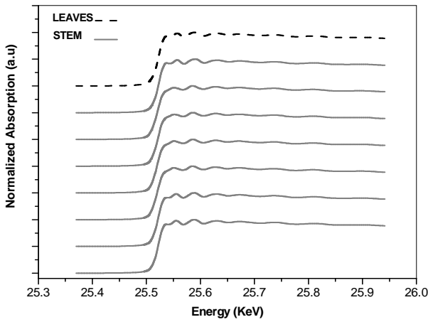
Fig. 2. Absorption spectra of stem and leaves samples which grew in cotton.
