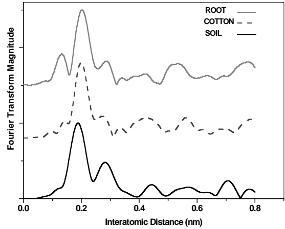
Fig. 4. Fourier transform of culture media (cotton and soil) and roots.
