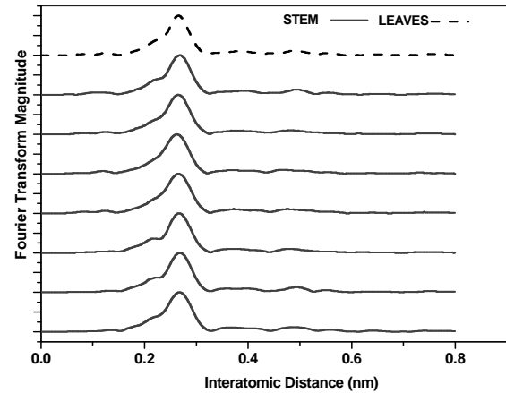
Fig. 5. Fourier transform of leaves and stems of plants grown in cotton.
