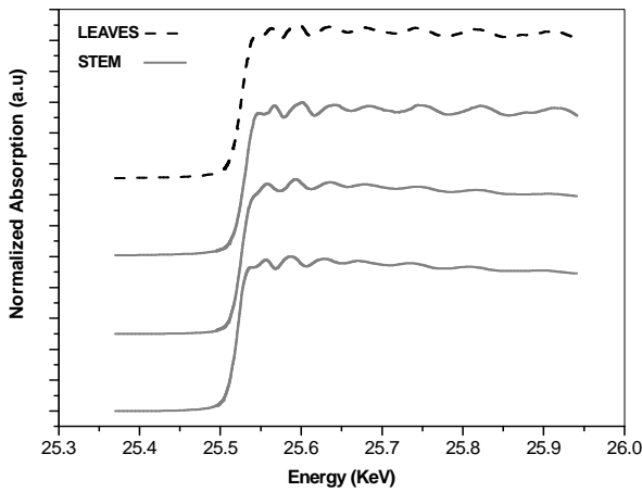
Fig. 3. Absorption spectra of stem and leaves samples which grew in soil.
