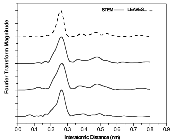
Fig. 6. Fourier transform of leaves and stems of plants grown in soil.
