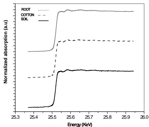
Fig. 1. Absorption spectra of culture media, (soil and cotton) and roots of plants.
