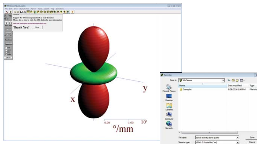
Figure 4: Screenshot of the Wintensor™ program displaying the longitudinal representation surface of the rotational power (optical activity) of \alpha -quartz. The monochrome point group of the physical property is \infty 2 , which allows for clockwise and anticlockwise rotations and is a supergroup of 32. The user can choose to convert the displayed model to either the *.stl or the *.wrl format, as documented by the inset to the right.
