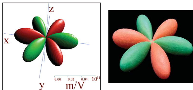
Figure 6: Longitudinal representation surface of the linear electro-optical (Pockels) effect in \alpha -quartz (left) as cropped from a screenshot of the Wintensor TM program and the corresponding 3D print out (right). The size of the 3D printed model is such that the 3.3 cm length of any one of the three positive (green) and three negative (red) lobes corresponds to 0.48 pm/V.
