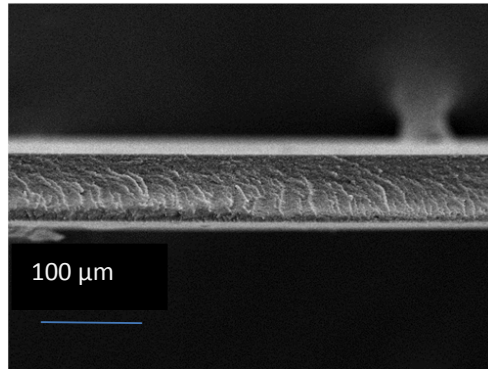
Figure 3. Scanning electron micrograph of membranes manufactured by acetylated cellulose of Pinus spp. saw dust.
