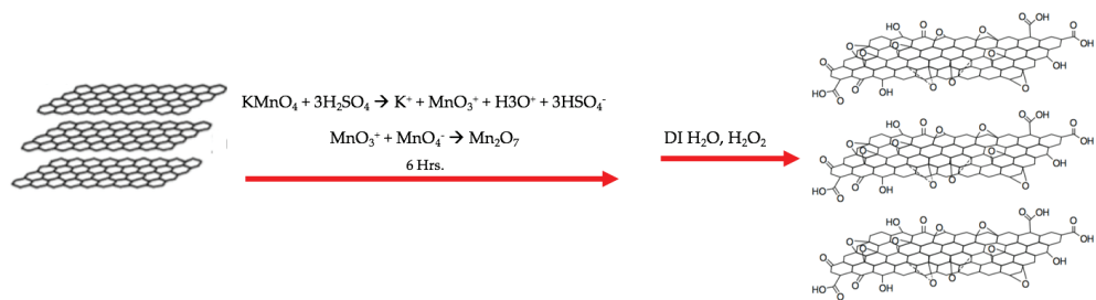
Figure 3. Chemical oxidation in Hummers' method [4].
