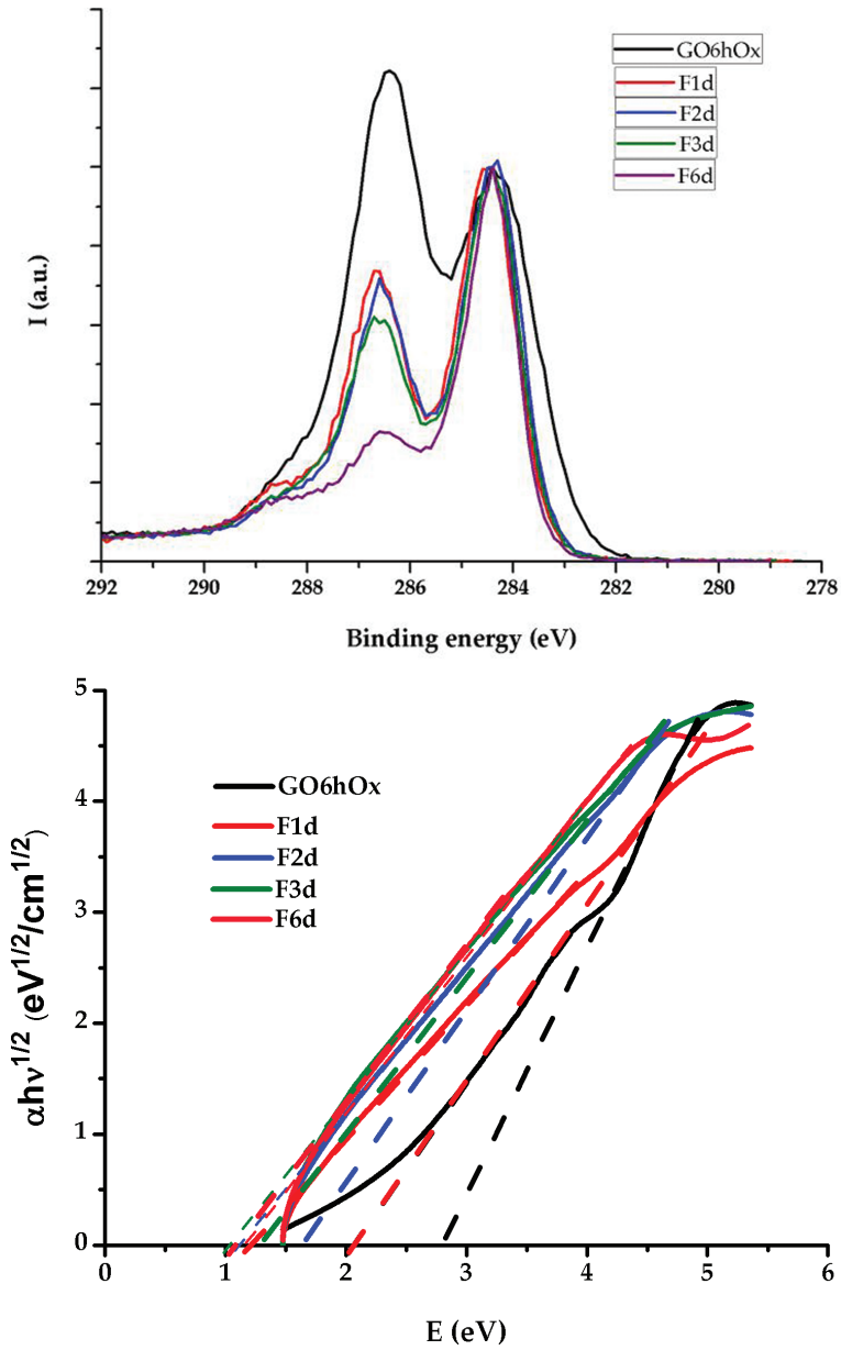
Figure 15. XPS C1s and Tauc plots for reduced graphene oxide with fructose. [2]
