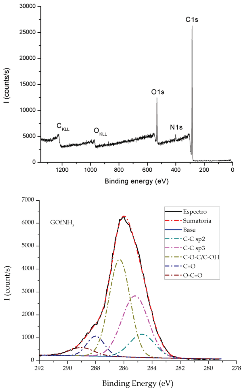
Figure 12. XPS survey and High resolution C1s of reduced graphene oxide functionalized with ODA [12].
