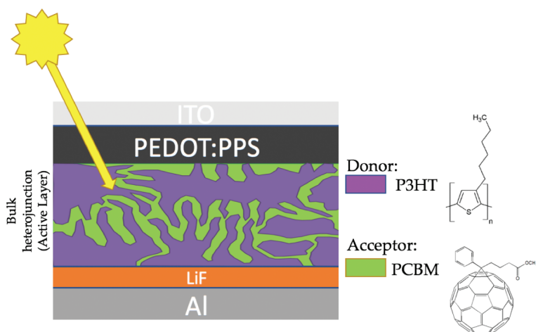
Figure 2. Typical diagram of an OPV-BHJ [12].
