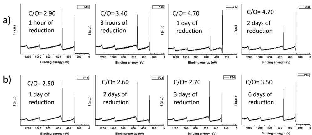
Figure 7. XPS survey of (a) GO with variable degrees of oxidation reduced with fructose; (b) reduced with ascorbic.
