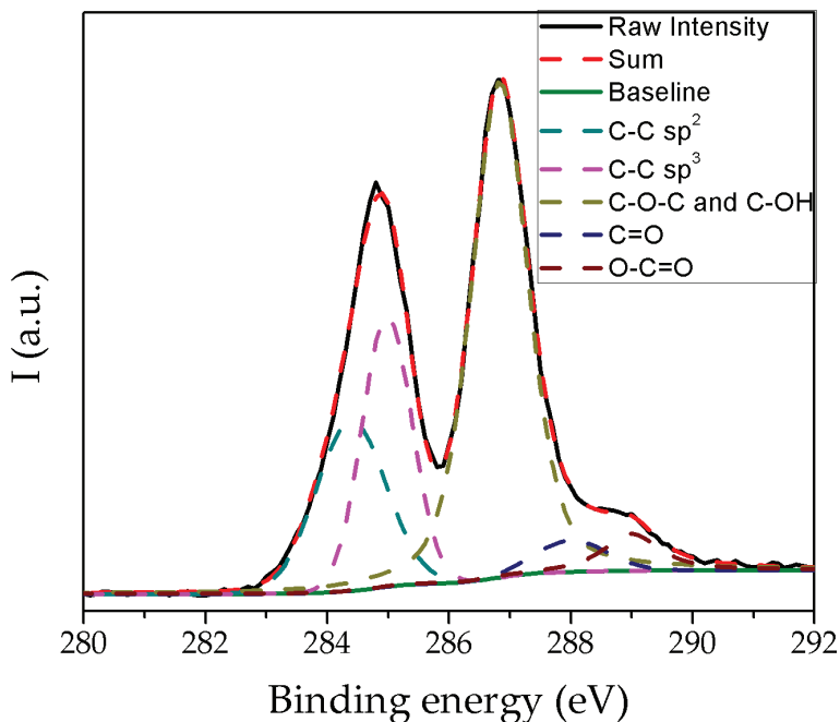
Figure 5. XPS for C1s [2].
