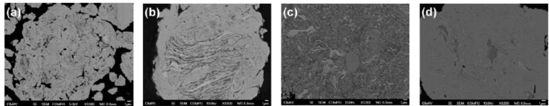
Fig. 1. Lamellar microstructure of mechanical alloyed powders, (a) NiCoAlFe, (b) NiCoAlFeCr, (c) NiCoAlFeTi and (d) NiCoAlFeCrTi systems.
