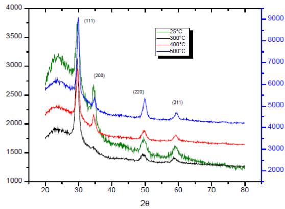
Fig. 1 XRD patterns of the 8 YSZ films prepared by sputtering onto glass at different temperatures.
