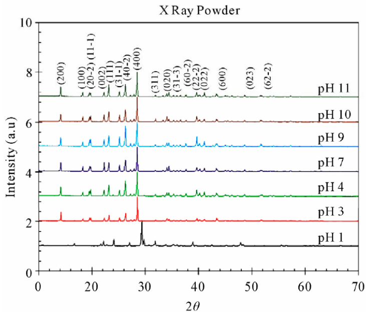
Figure 3. The X-ray pattern for GSN at different pH.
