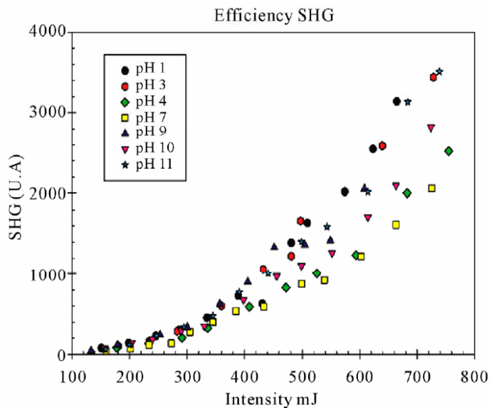
Figure 4. The SHG signal of GSN at different pH.
