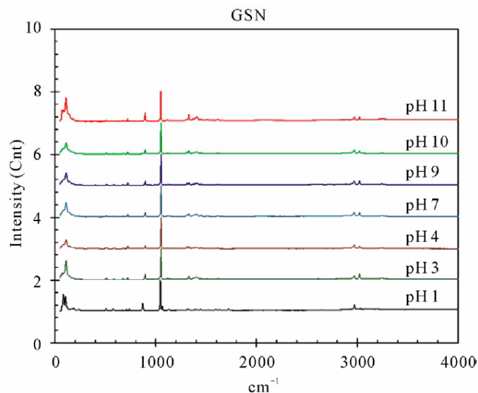
Figure 2. The RAMAN spectra of GSN at different pH.
