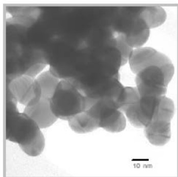
Fig. 7. Ag Nanoparticles in leaves.
